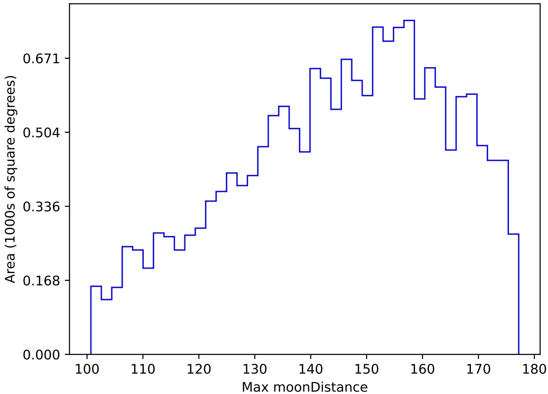
ddf_loaded_fl4_v3.4_10yrs WFD y band: Max moonDistance
