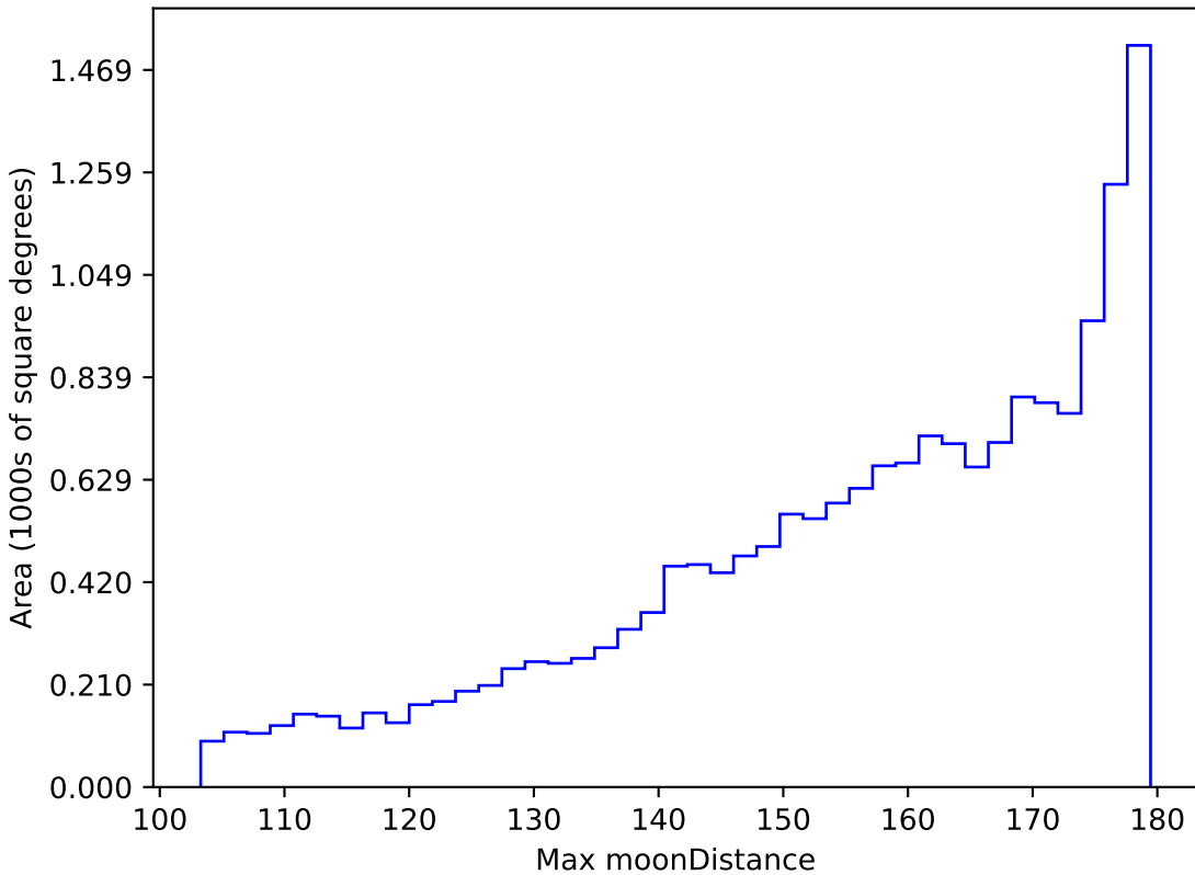
ddf_loaded_fl4_v3.4_10yrs WFD r band: Max moonDistance
