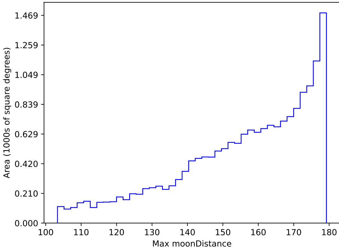
ddf_loaded_fl4_v3.4_10yrs WFD i band: Max moonDistance
