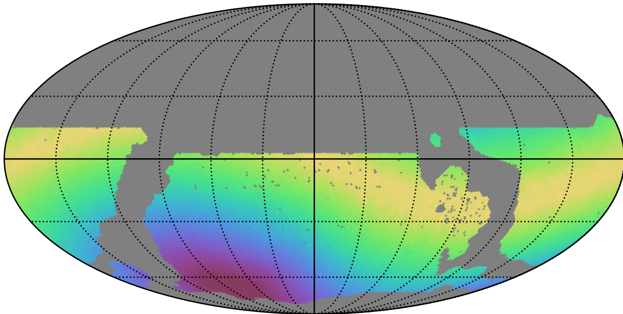
ddf_loaded_fl4_v3.4_10yrs WFD all bands: Max moonDistance
