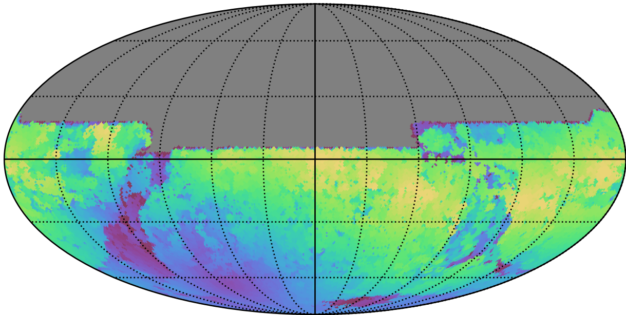
ddf_loaded_fl4_v3.4_10yrs All sky y band: Max moonDistance
