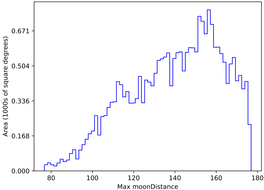
ddf_loaded_fl4_v3.4_10yrs All sky y band: Max moonDistance
