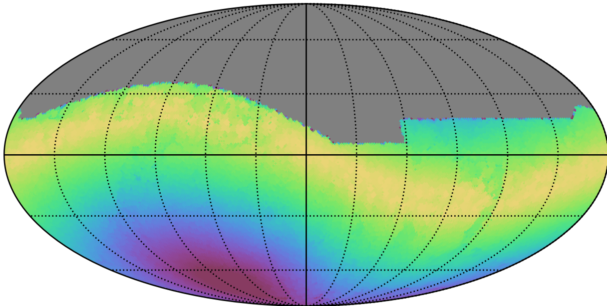
ddf_loaded_fl4_v3.4_10yrs All sky r band: Max moonDistance
