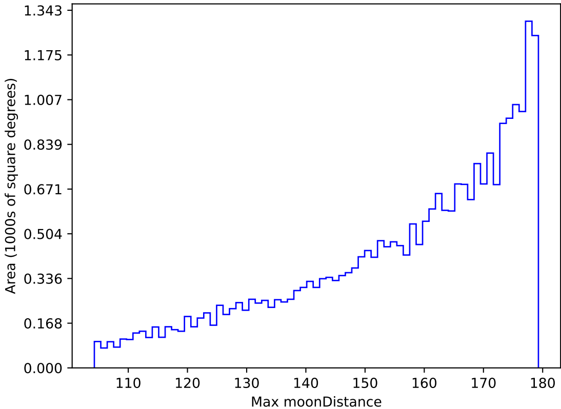
ddf_loaded_fl4_v3.4_10yrs All sky r band: Max moonDistance
