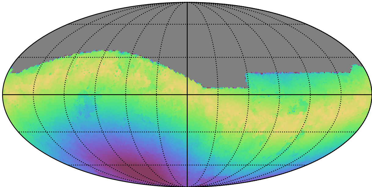
ddf_loaded_fl4_v3.4_10yrs All sky g band: Max moonDistance
