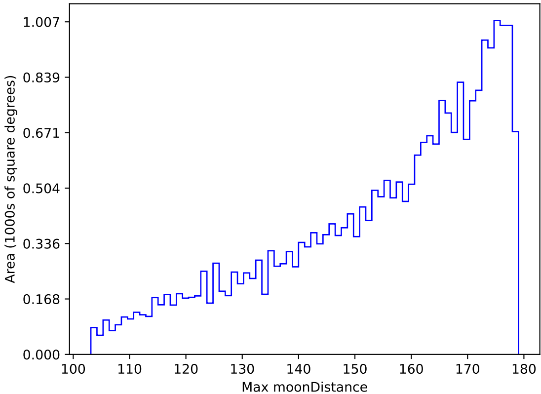
ddf_loaded_fl4_v3.4_10yrs All sky g band: Max moonDistance
