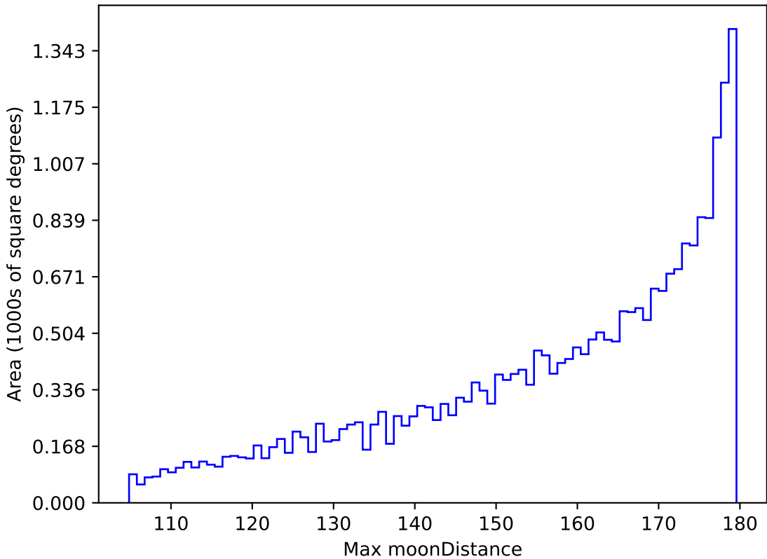
ddf_loaded_fl4_v3.4_10yrs All sky all bands: Max moonDistance
