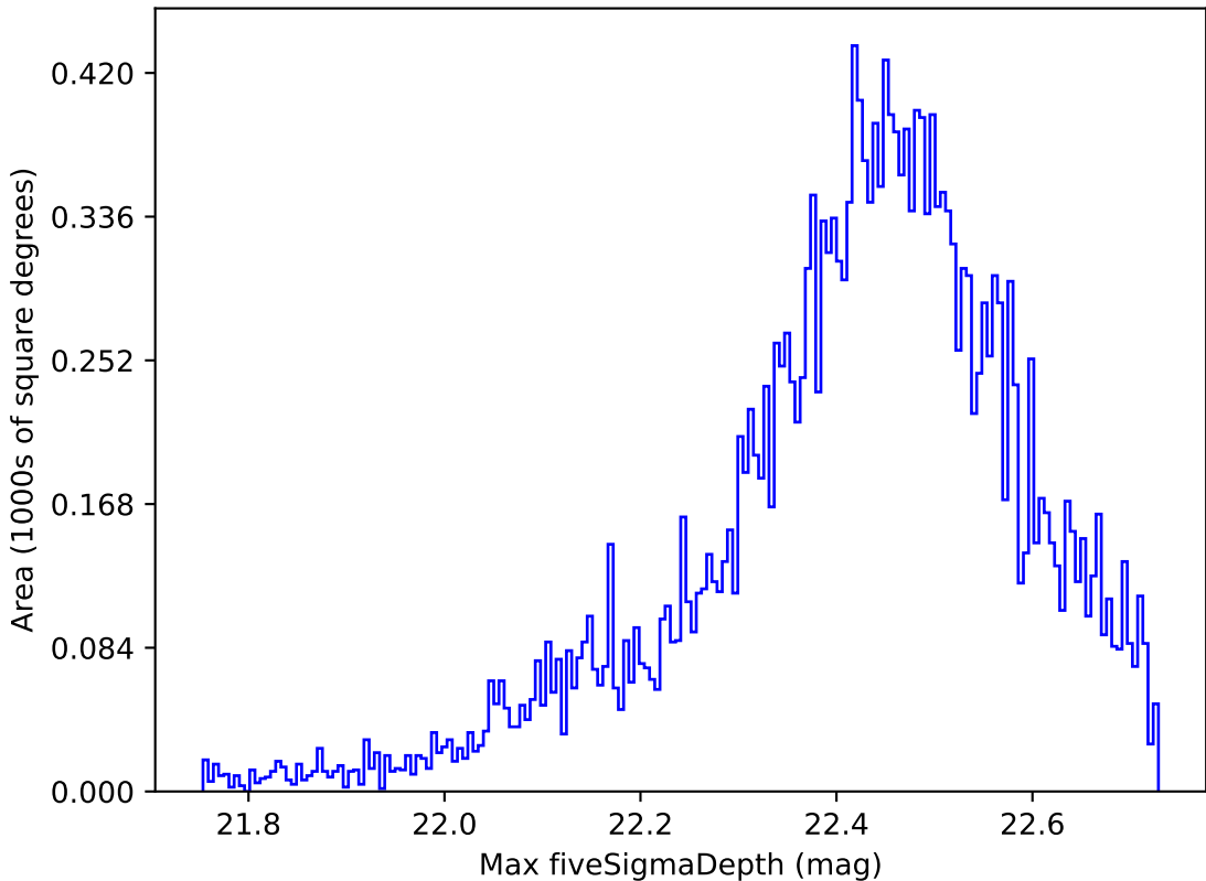
ddf_loaded_fl4_v3.4_10yrs Yr 1 y band: Max fiveSigmaDepth
