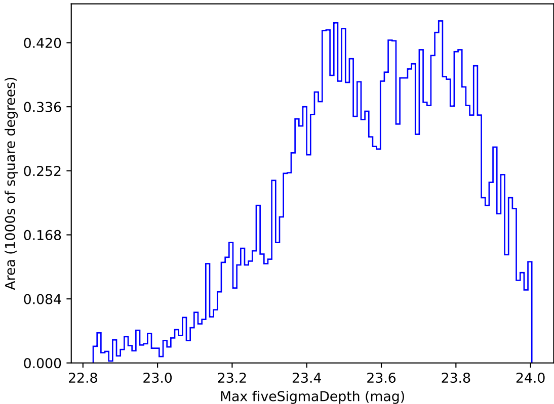
ddf_loaded_fl4_v3.4_10yrs Yr 1 u band: Max fiveSigmaDepth
