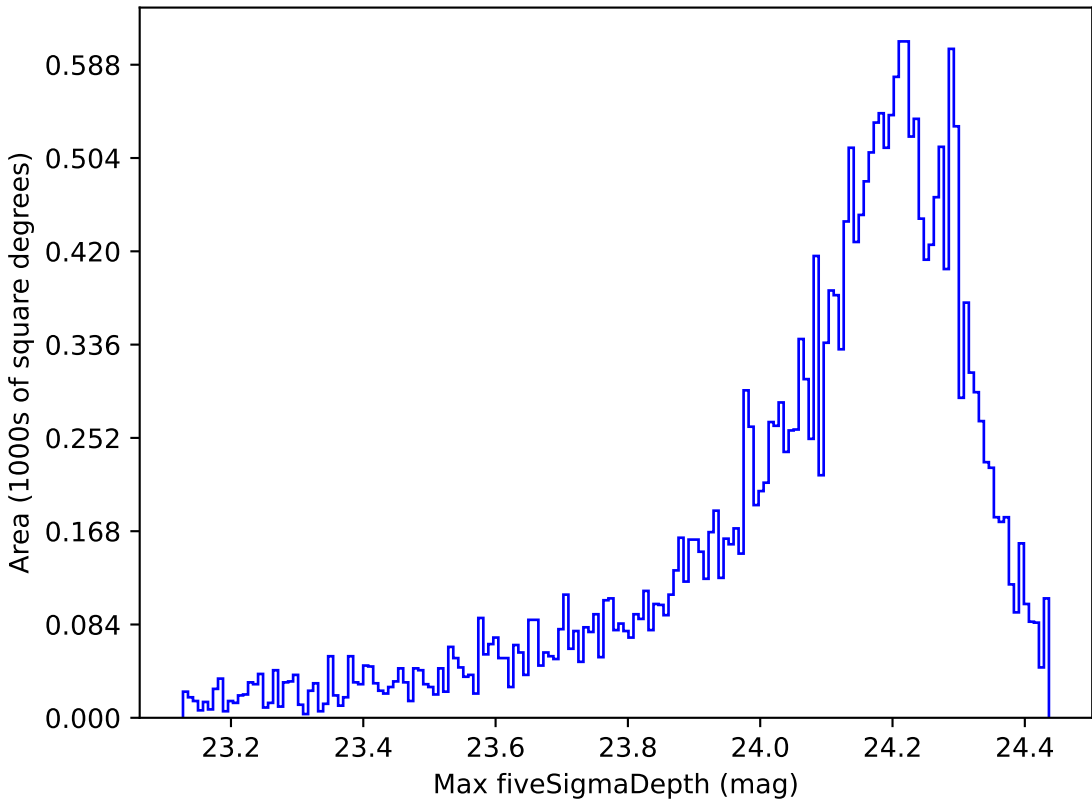
ddf_loaded_fl4_v3.4_10yrs Yr 1 i band: Max fiveSigmaDepth
