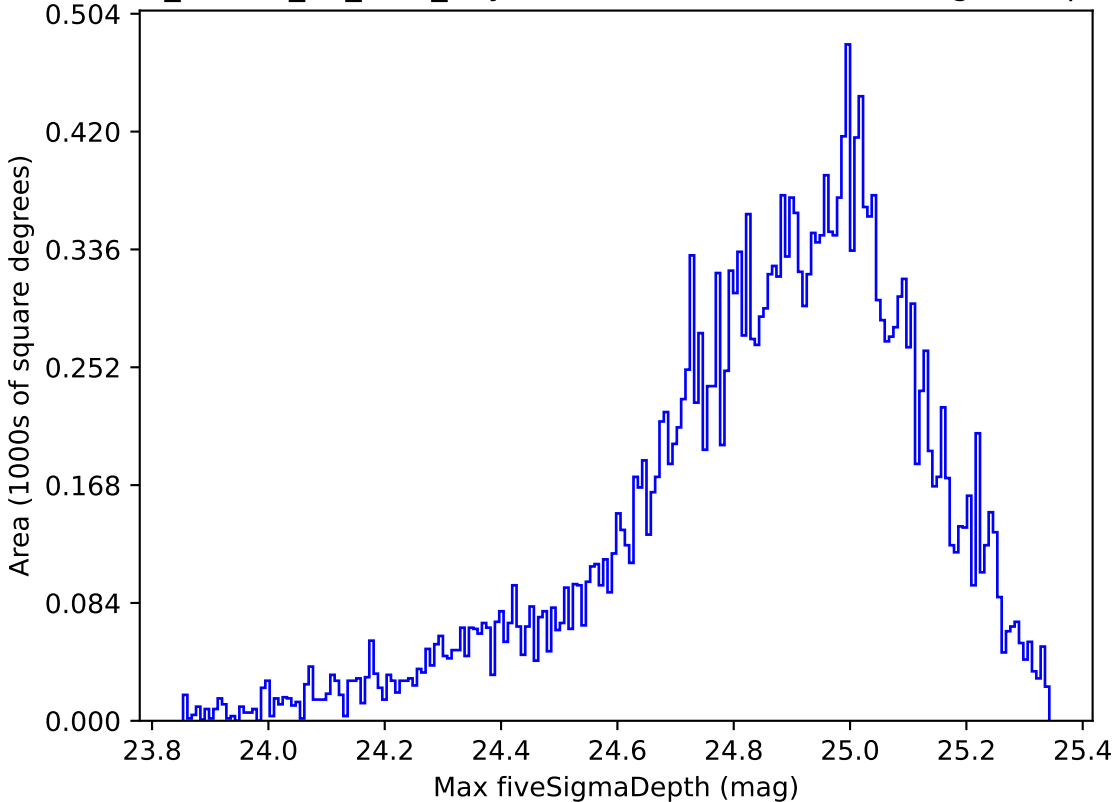
ddf_loaded_fl4_v3.4_10yrs Yr 1 all bands: Max fiveSigmaDepth
