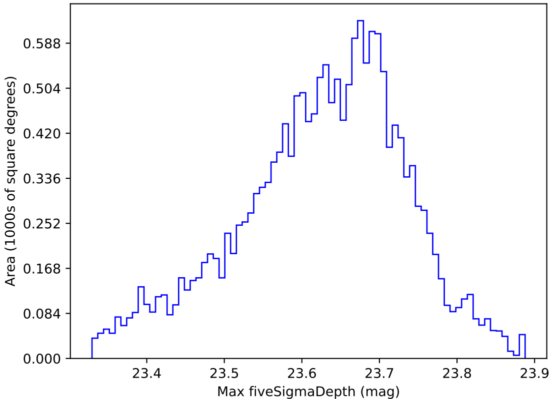
ddf_loaded_fl4_v3.4_10yrs WFD z band: Max fiveSigmaDepth
