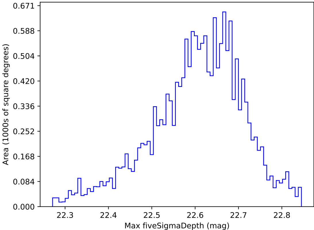
ddf_loaded_fl4_v3.4_10yrs WFD y band: Max fiveSigmaDepth
