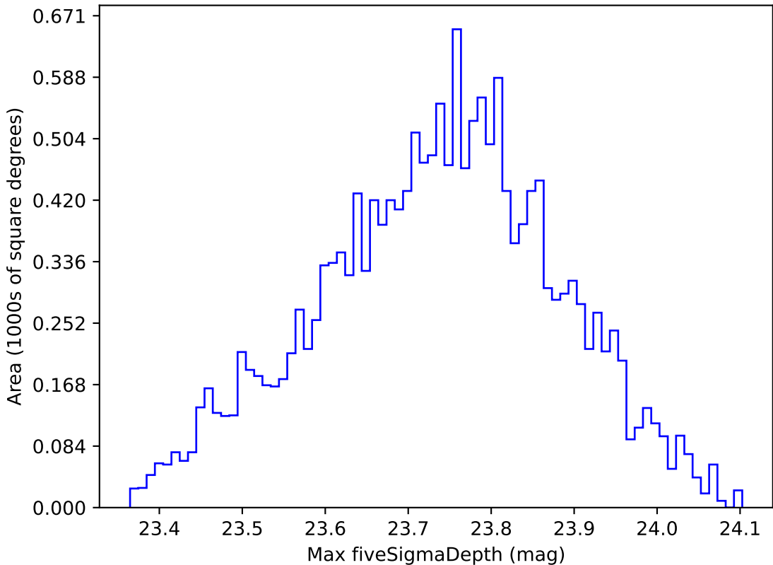
ddf_loaded_fl4_v3.4_10yrs WFD u band: Max fiveSigmaDepth
