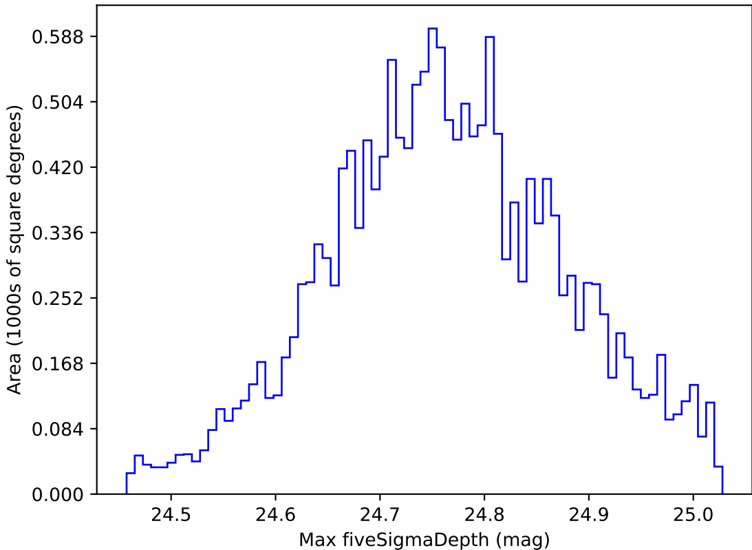
ddf_loaded_fl4_v3.4_10yrs WFD r band: Max fiveSigmaDepth
