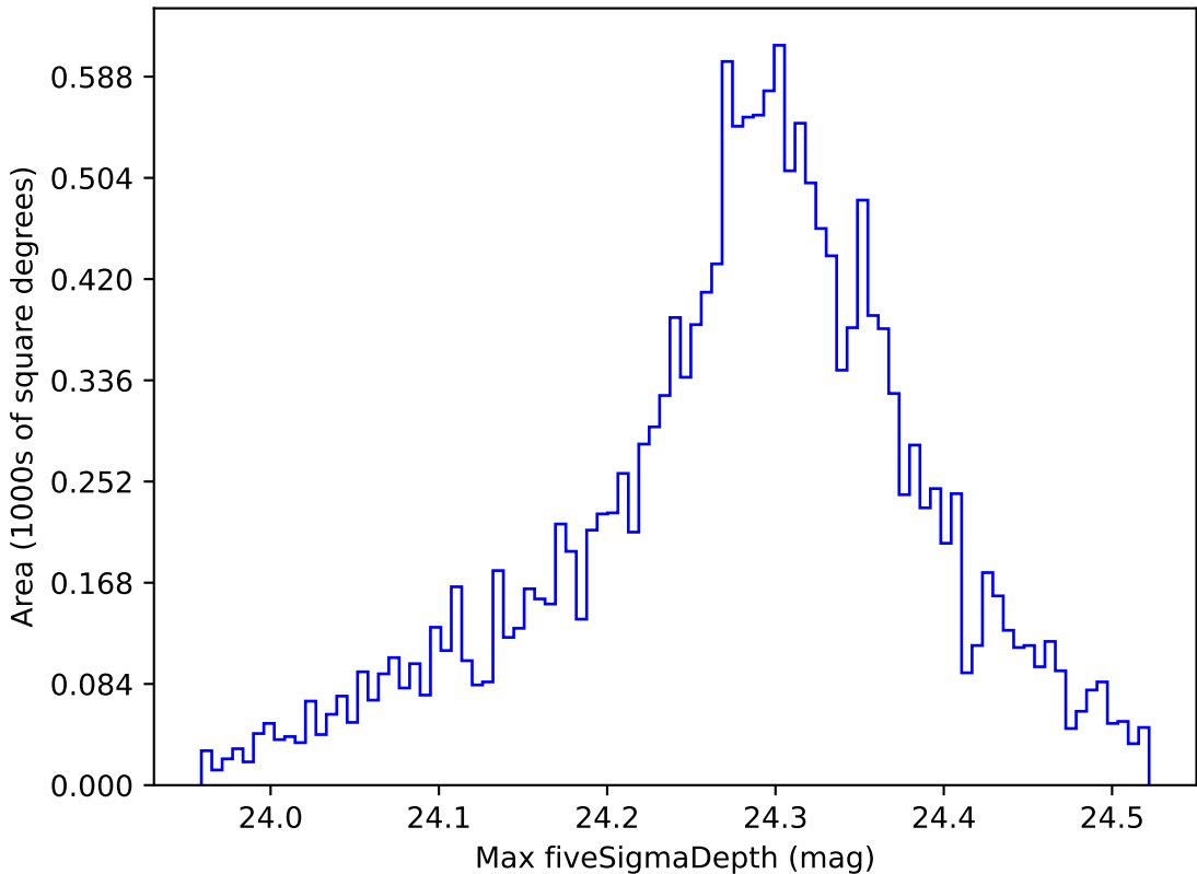
ddf_loaded_fl4_v3.4_10yrs WFD i band: Max fiveSigmaDepth
