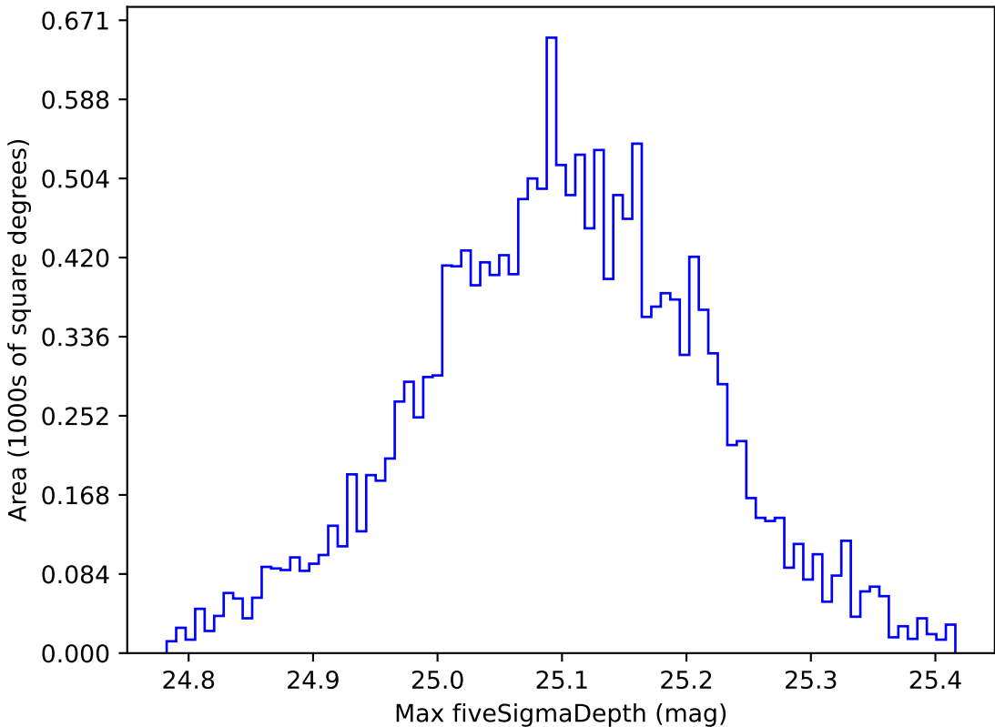
ddf_loaded_fl4_v3.4_10yrs WFD g band: Max fiveSigmaDepth
