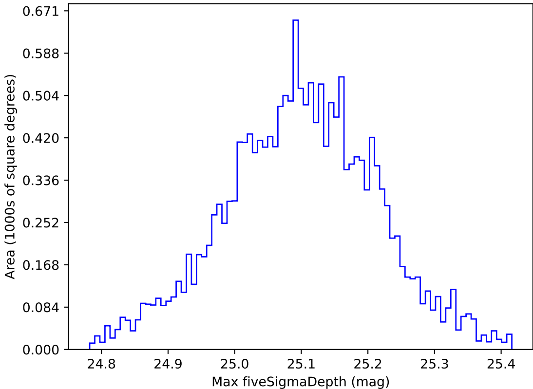
ddf_loaded_fl4_v3.4_10yrs WFD all bands: Max fiveSigmaDepth
