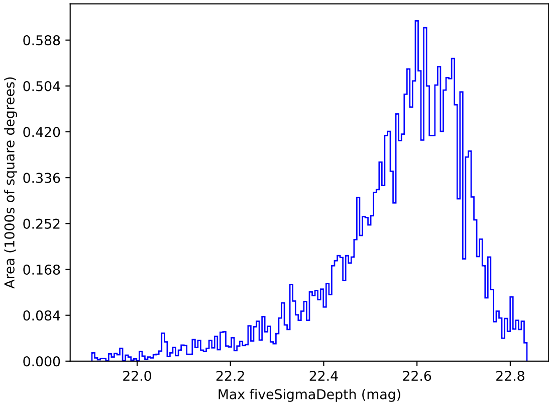
ddf_loaded_fl4_v3.4_10yrs All sky y band: Max fiveSigmaDepth
