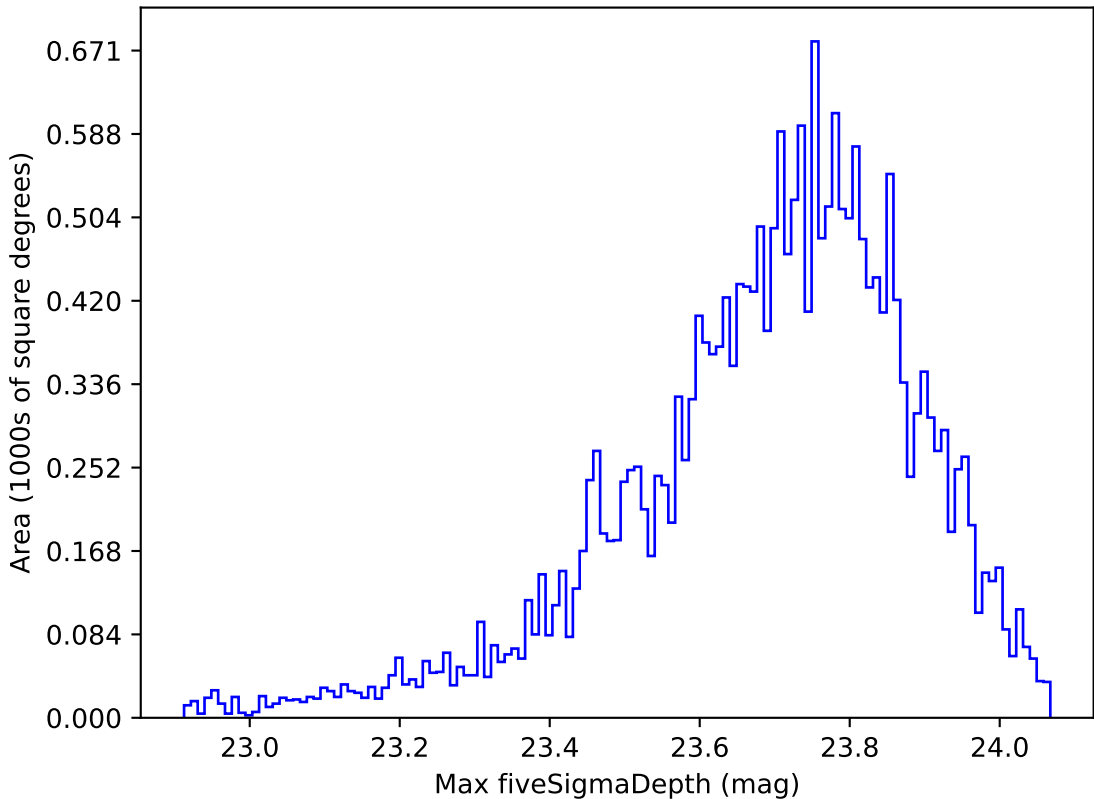
ddf_loaded_fl4_v3.4_10yrs All sky u band: Max fiveSigmaDepth
