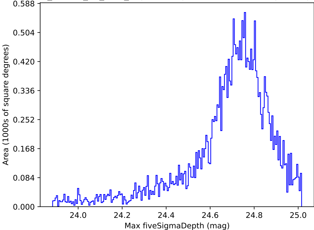
ddf_loaded_fl4_v3.4_10yrs All sky r band: Max fiveSigmaDepth
