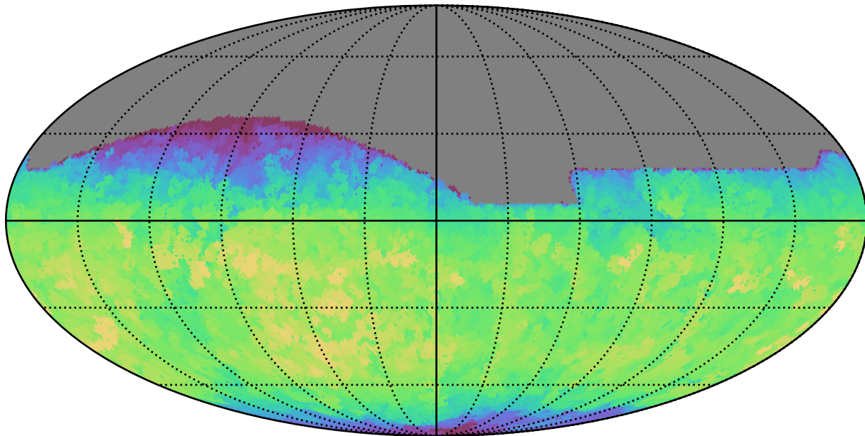
ddf_loaded_fl4_v3.4_10yrs All sky i band: Max fiveSigmaDepth
