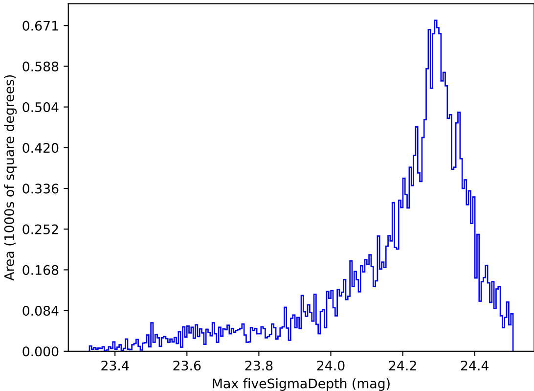
ddf_loaded_fl4_v3.4_10yrs All sky i band: Max fiveSigmaDepth
