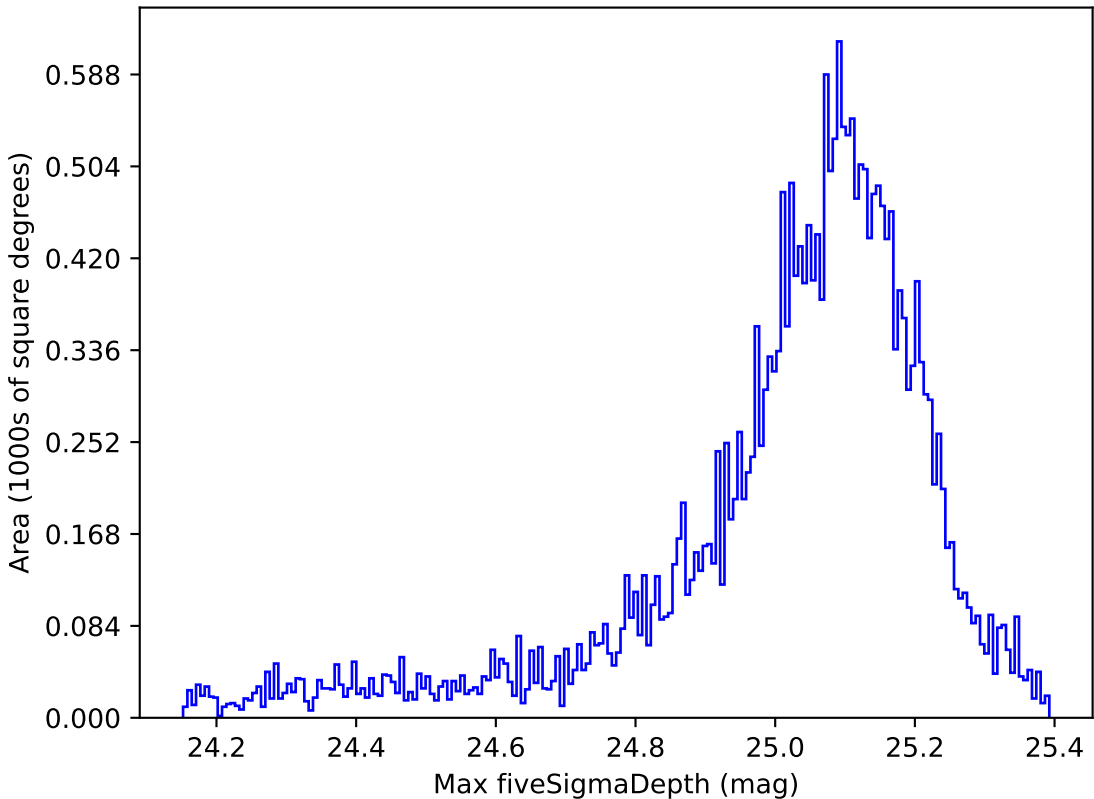
ddf_loaded_fl4_v3.4_10yrs All sky g band: Max fiveSigmaDepth
