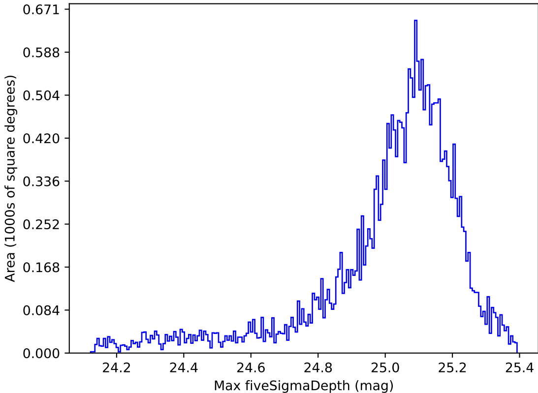
ddf_loaded_fl4_v3.4_10yrs All sky all bands: Max fiveSigmaDepth
