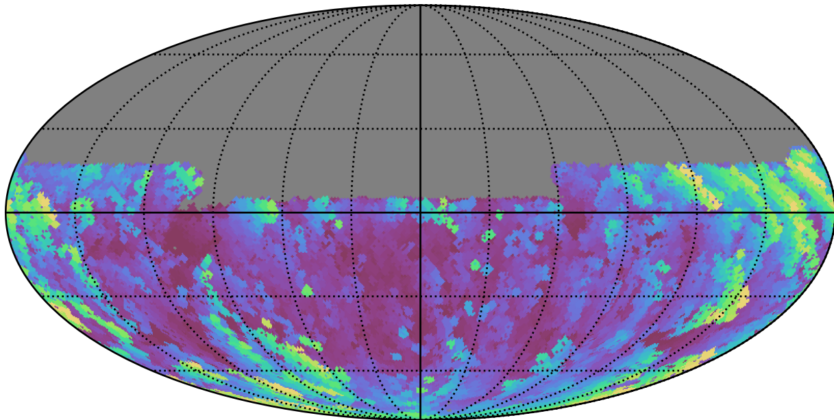
ddf_loaded_fl4_v3.4_10yrs Yr 1 y band: Max airmass
