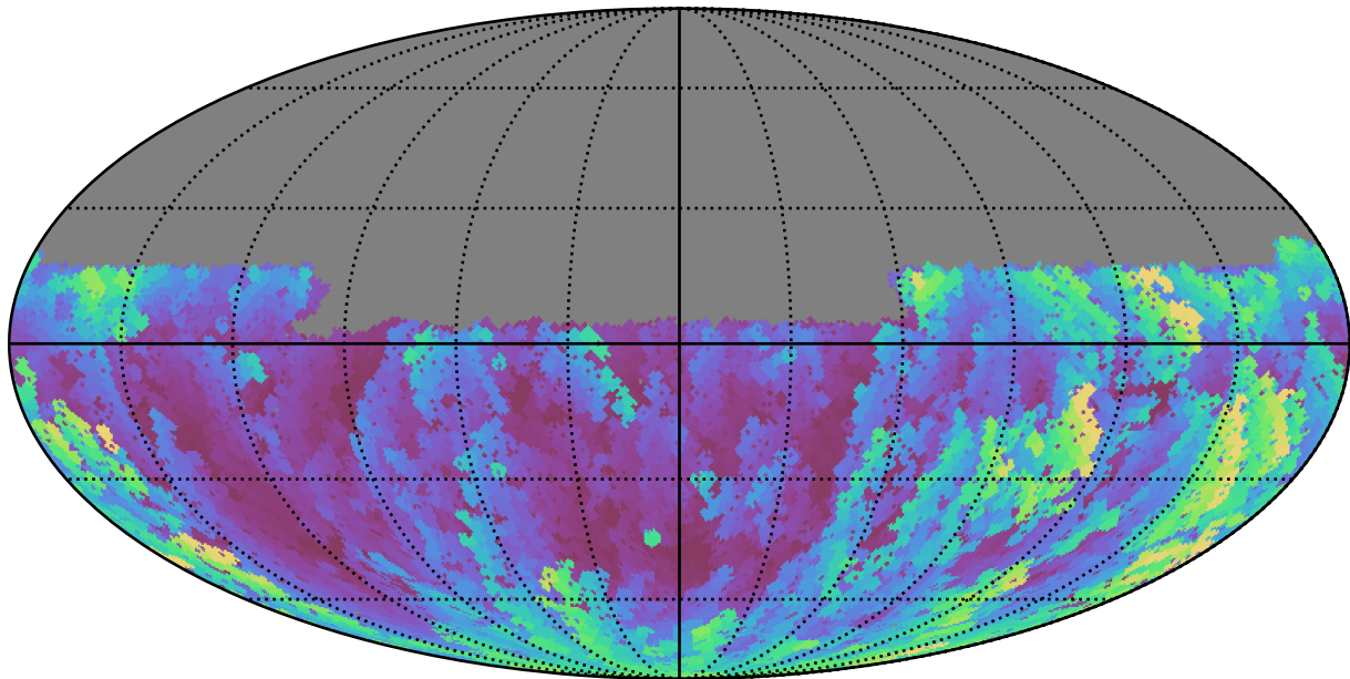
ddf_loaded_fl4_v3.4_10yrs Yr 1 u band: Max airmass
