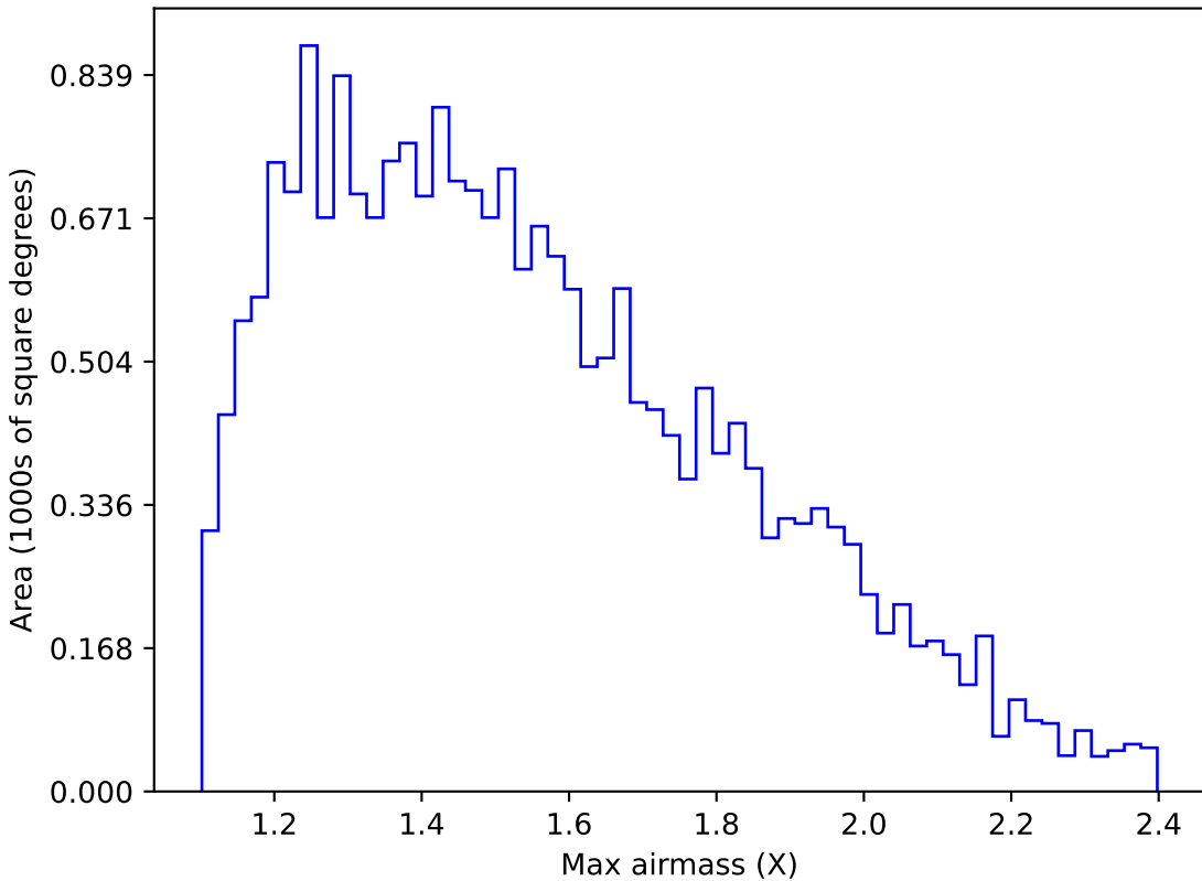
ddf_loaded_fl4_v3.4_10yrs Yr 1 u band: Max airmass
