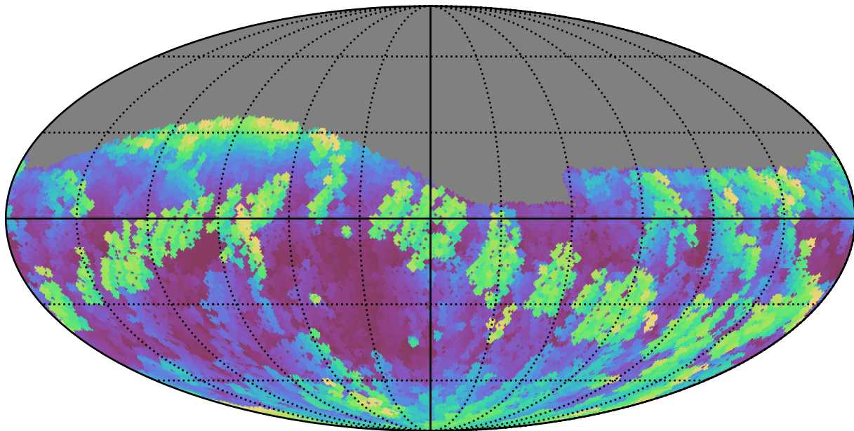
ddf_loaded_fl4_v3.4_10yrs Yr 1 r band: Max airmass
