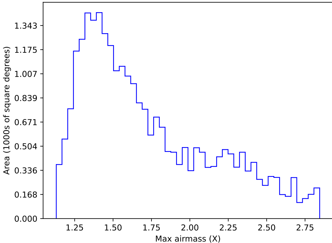
ddf_loaded_fl4_v3.4_10yrs Yr 1 i band: Max airmass
