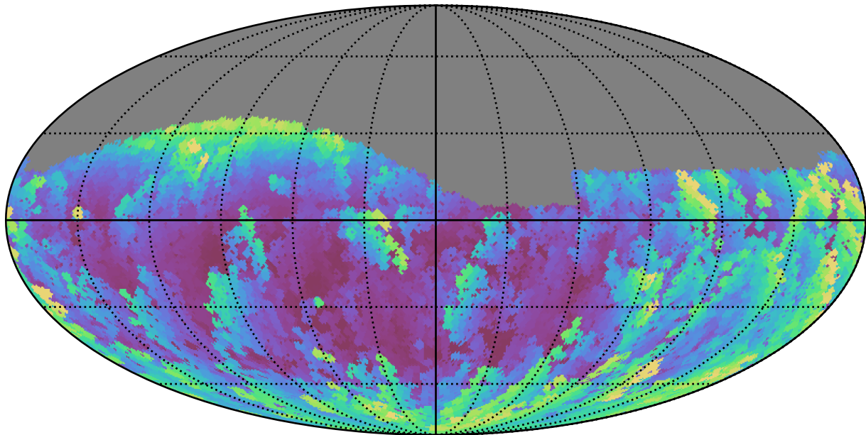
ddf_loaded_fl4_v3.4_10yrs Yr 1 g band: Max airmass
