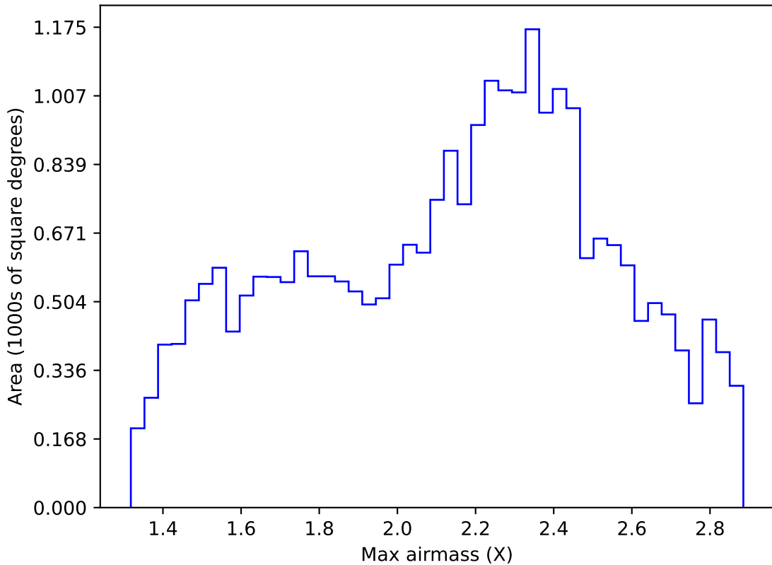
ddf_loaded_fl4_v3.4_10yrs Yr 1 all bands: Max airmass
