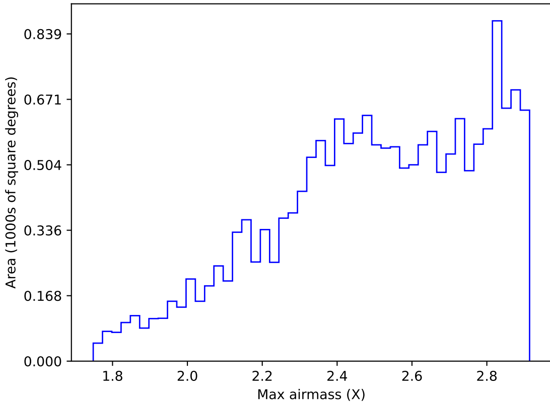
ddf_loaded_fl4_v3.4_10yrs WFD z band: Max airmass
