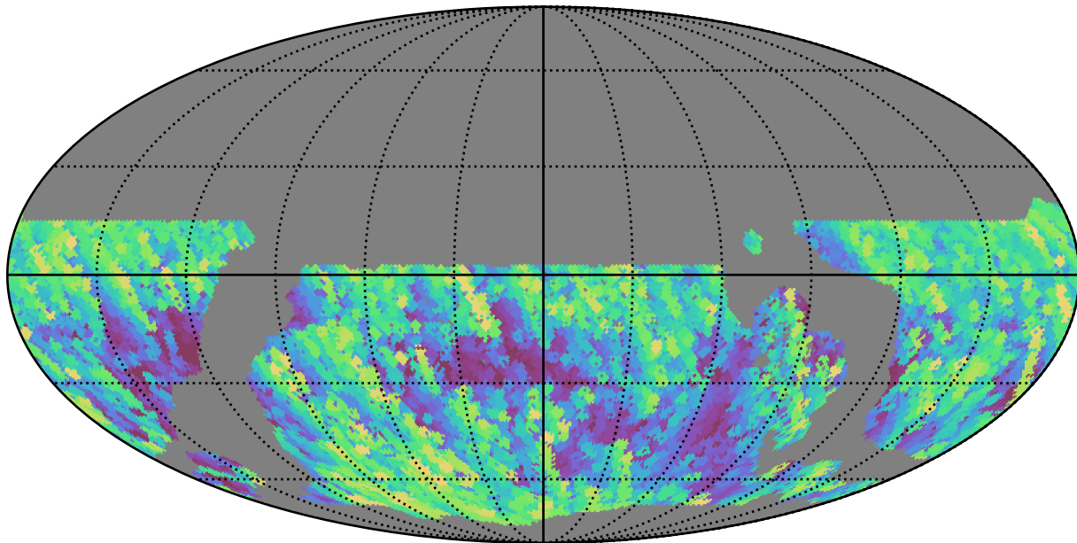
ddf_loaded_fl4_v3.4_10yrs WFD y band: Max airmass
