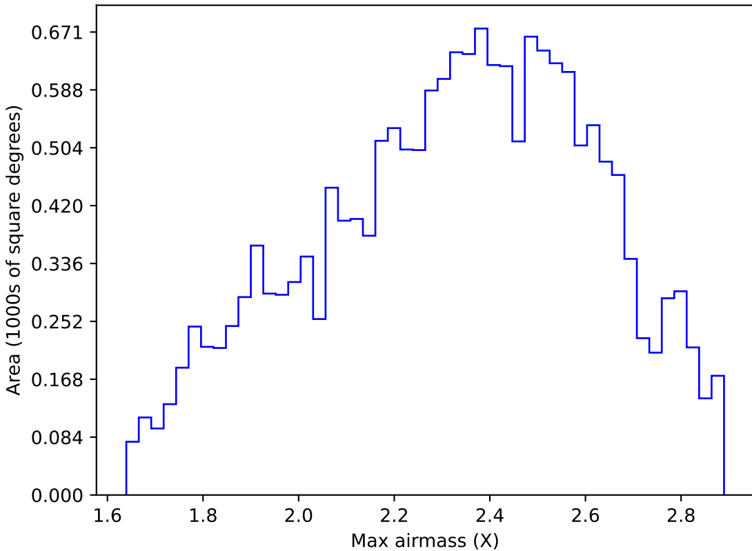
ddf_loaded_fl4_v3.4_10yrs WFD y band: Max airmass
