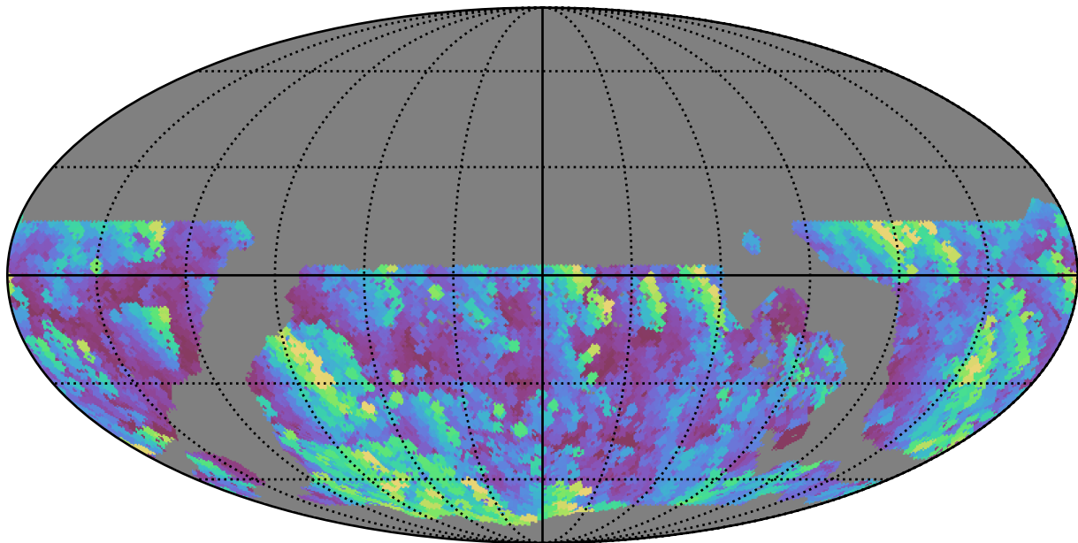
ddf_loaded_fl4_v3.4_10yrs WFD u band: Max airmass
