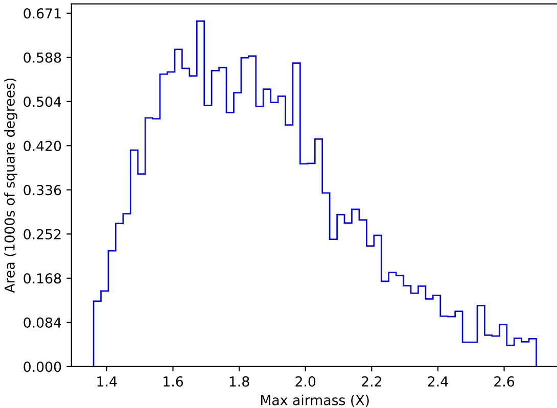
ddf_loaded_fl4_v3.4_10yrs WFD u band: Max airmass
