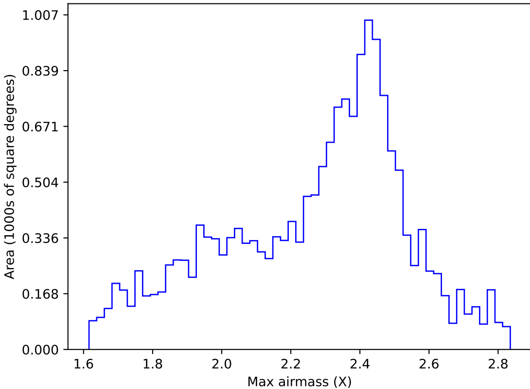
ddf_loaded_fl4_v3.4_10yrs WFD r band: Max airmass
