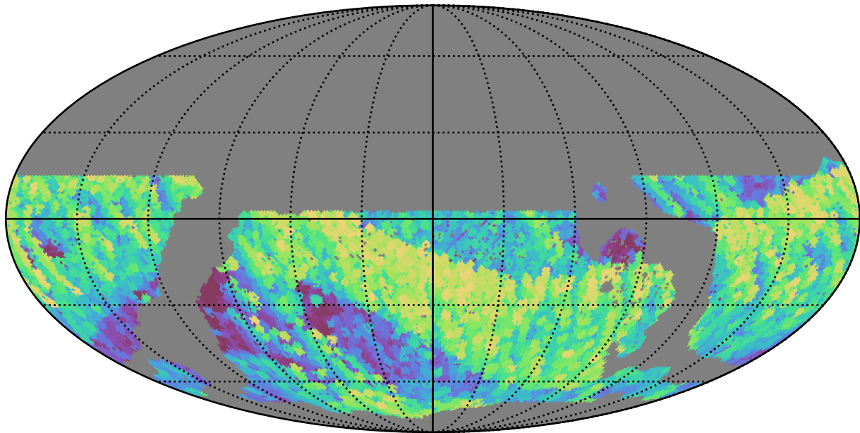
ddf_loaded_fl4_v3.4_10yrs WFD i band: Max airmass
