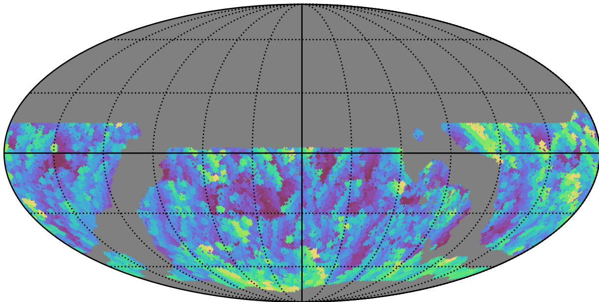
ddf_loaded_fl4_v3.4_10yrs WFD g band: Max airmass
