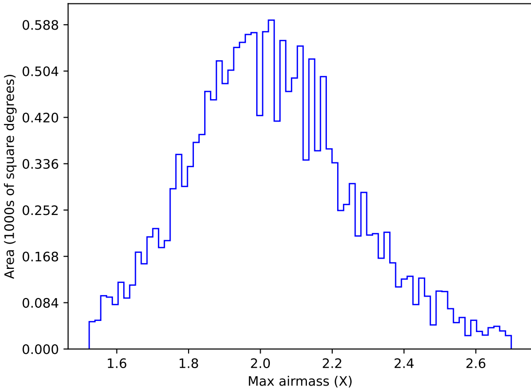
ddf_loaded_fl4_v3.4_10yrs WFD g band: Max airmass
