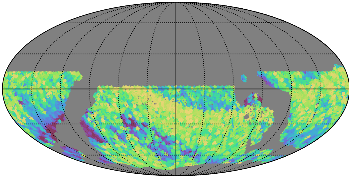
ddf_loaded_fl4_v3.4_10yrs WFD all bands: Max airmass
