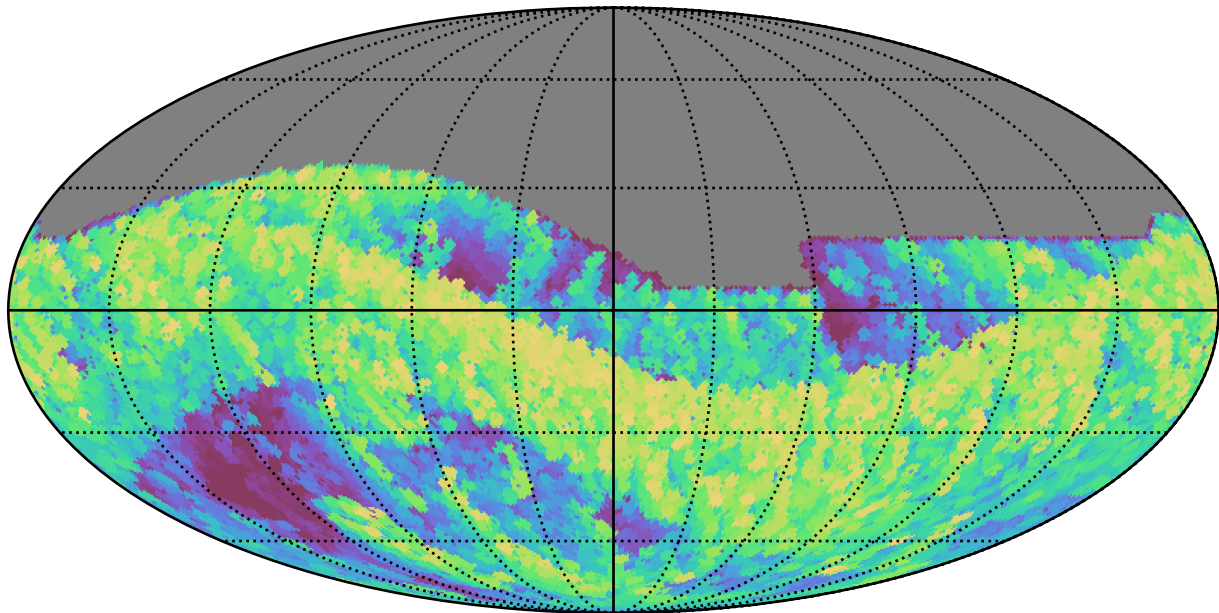
ddf_loaded_fl4_v3.4_10yrs All sky z band: Max airmass
