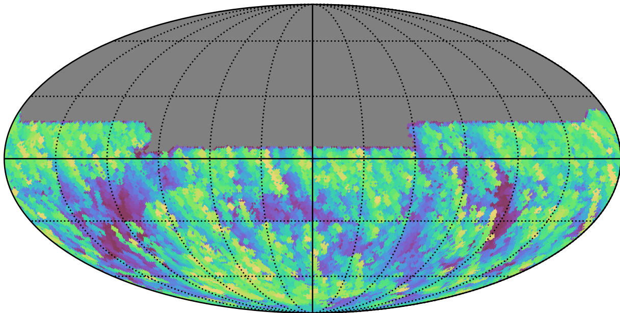
ddf_loaded_fl4_v3.4_10yrs All sky y band: Max airmass
