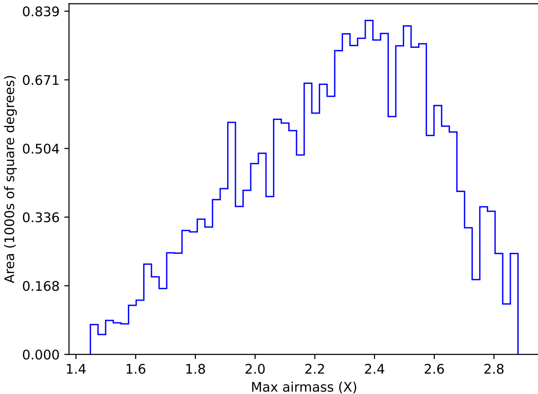
ddf_loaded_fl4_v3.4_10yrs All sky y band: Max airmass
