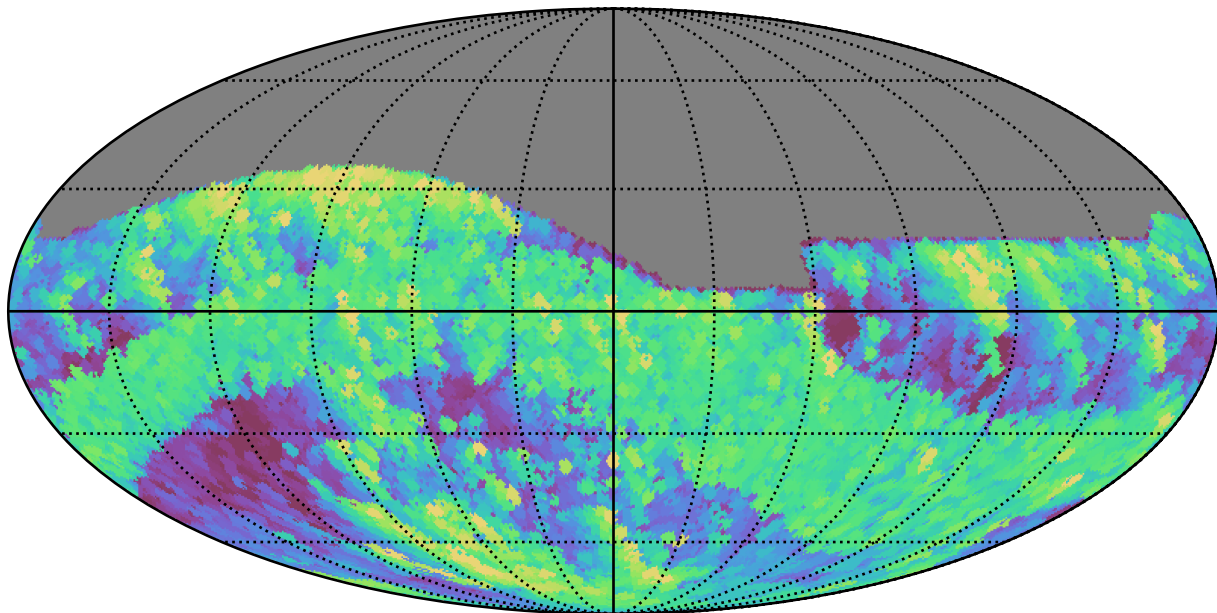
ddf_loaded_fl4_v3.4_10yrs All sky r band: Max airmass
